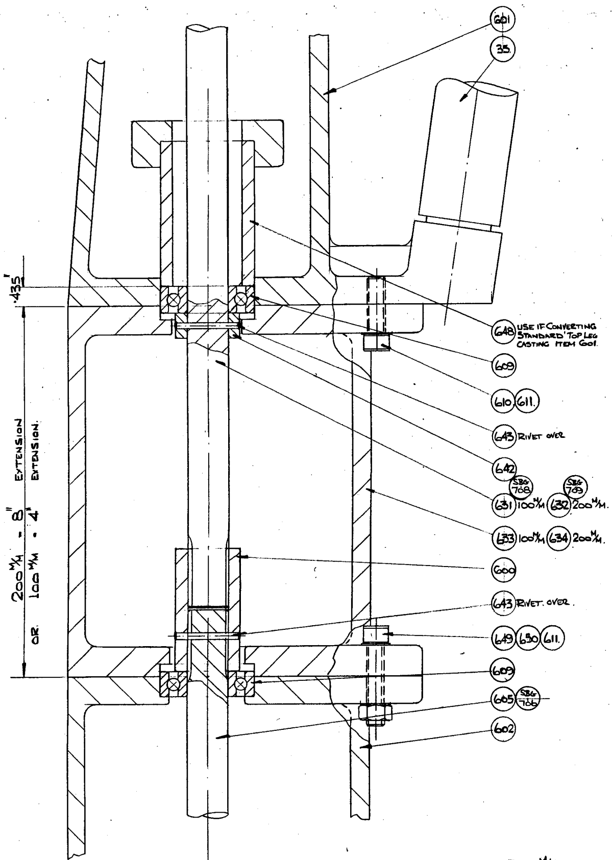
EXTENSION DETAIL FOR 900 MM TO 6096 AND 1000 MM . TYPE 2 CAT DRIVE.
